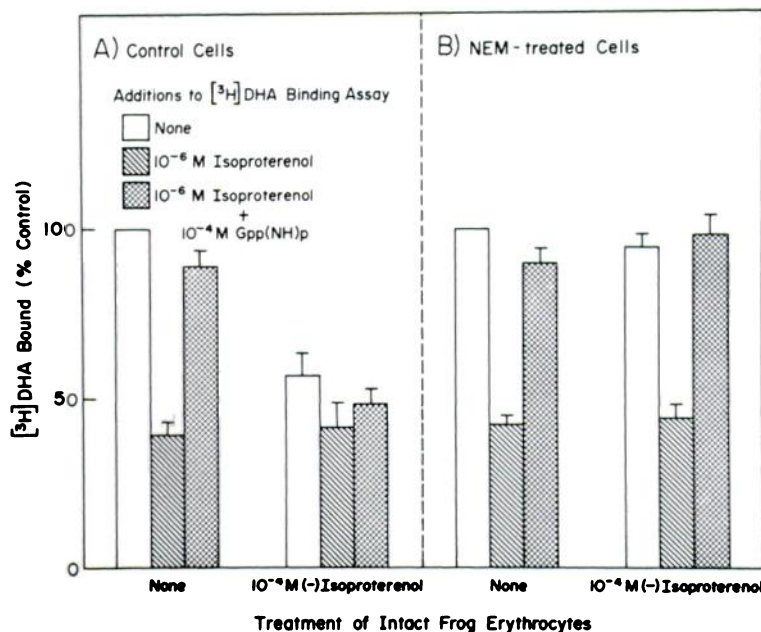
FIG. 4. Exposure of intact frog erythrocytes to NEM does not affect the ability of (-)-isoproterenol to form a nucleotide sensitive high affinity complex with beta-adrenergic receptors in erythrocyte membranes
