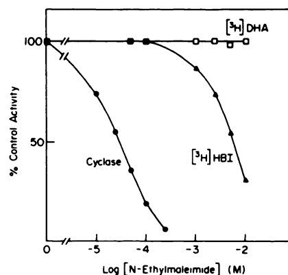
FIG. 1. Effect of NEM on adenylate cyclase activity and on the binding of [ ^3 H]DHA and [ ^3 H]HBI
