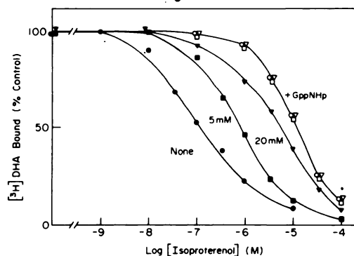
FIG. 2. (-)Isoproterenol competition for [ ^3 H]DHA binding to frog erythrocyte membranes pretreated with NEM
